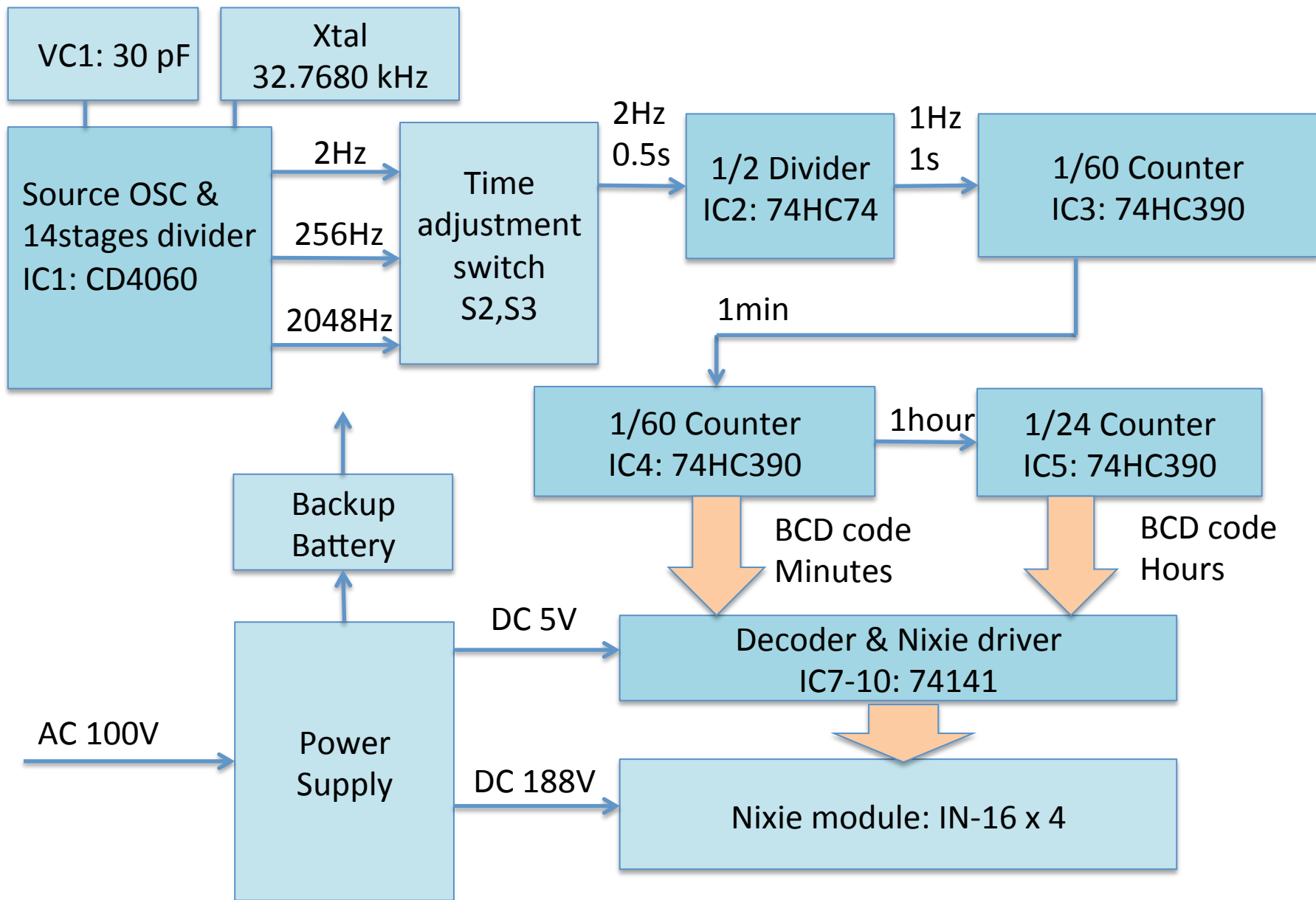
Fig 1 Nixie Clock block diagram
